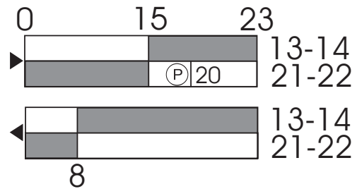
Switching diagram
